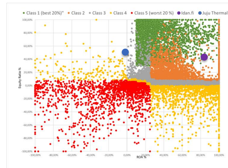
Logistic regression - based model
